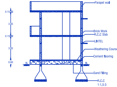
CROSS SECTION ON 'AB'
