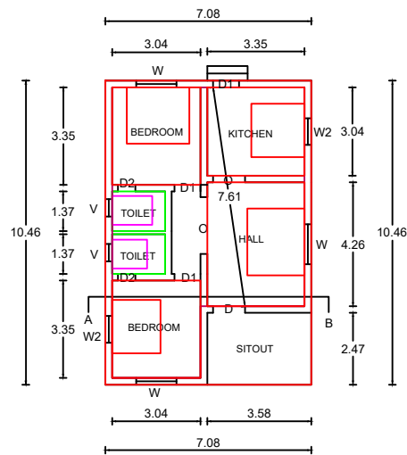
GROND FLOOR PLAN
