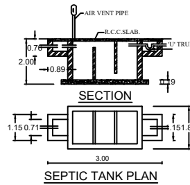
SECTION SEPTIC TANK PLAN
