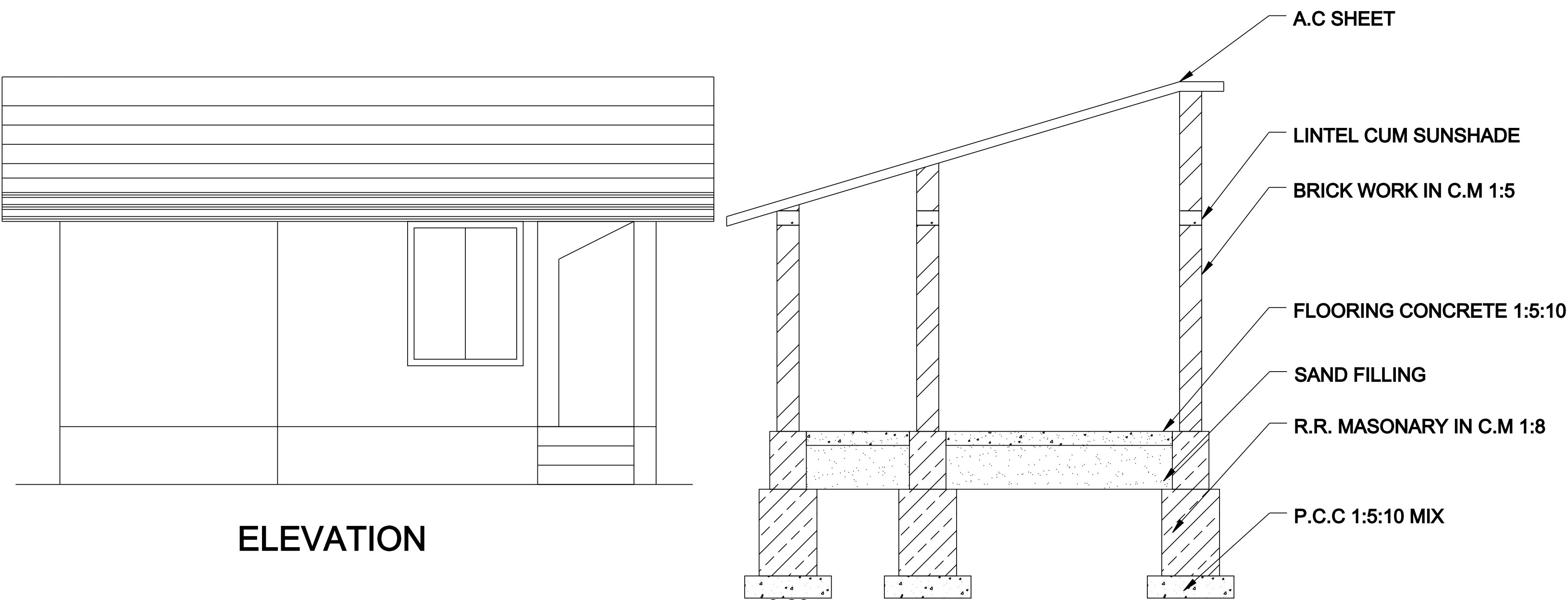
SECTION 'AA'
