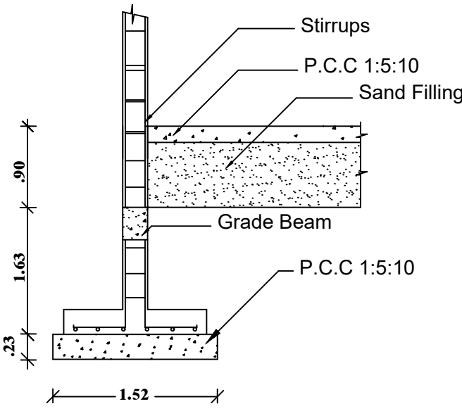
COLUMN DETAIL
