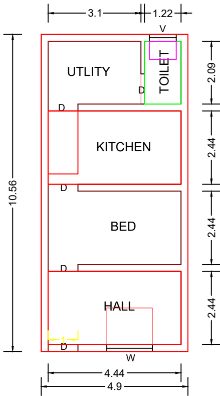
G.FLOOR PLAN
