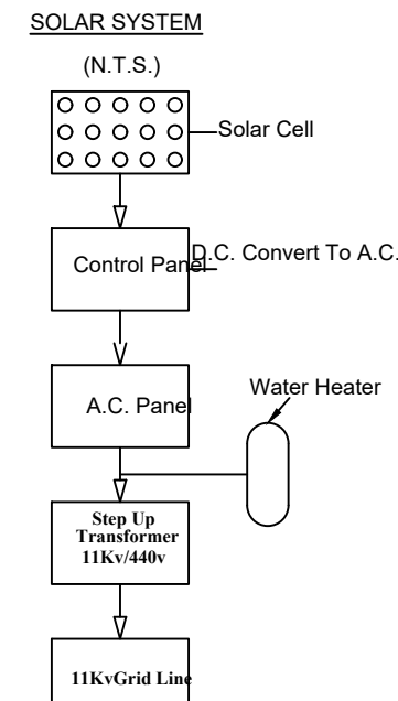
SOLAR SYSTEM FLOW DIAGRAM
