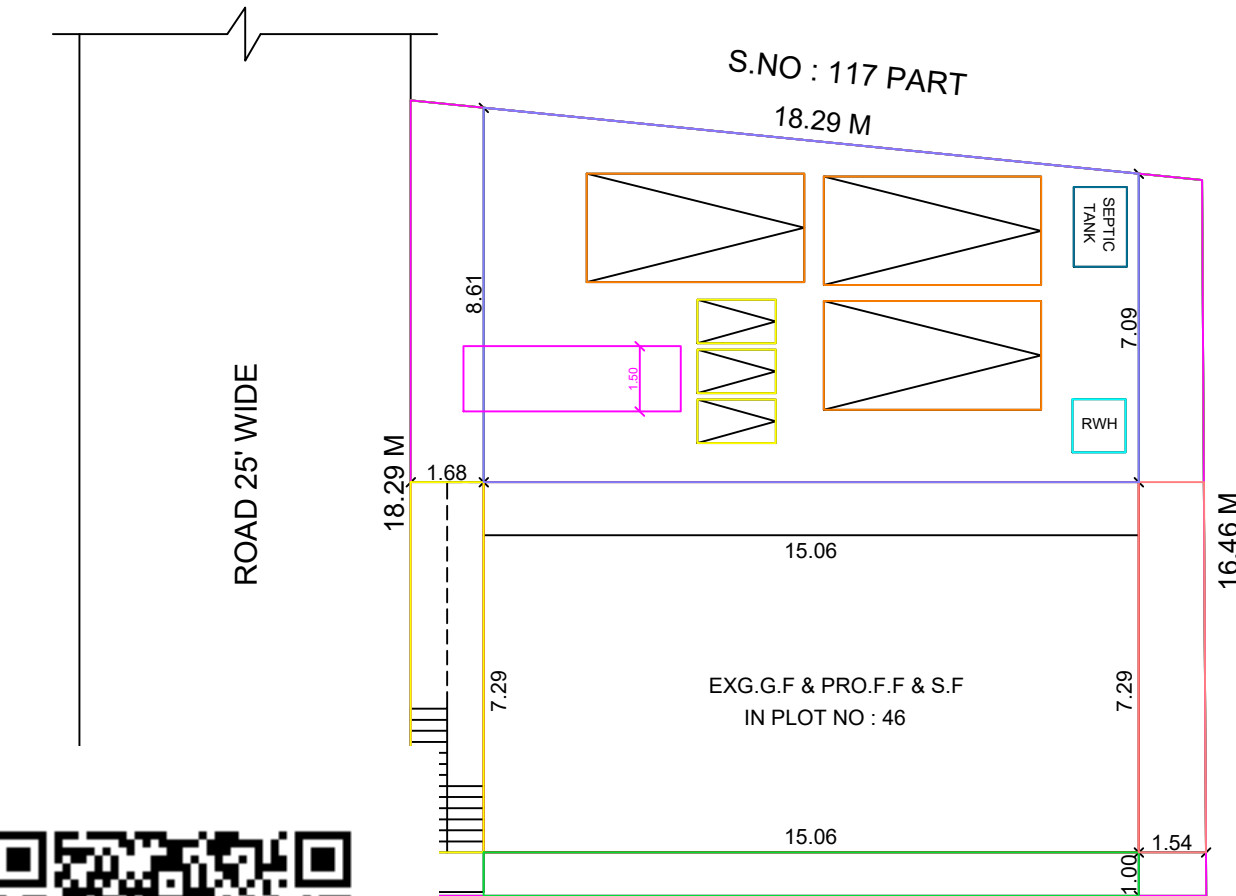
EXG.GROUND FLOOR PLAN
