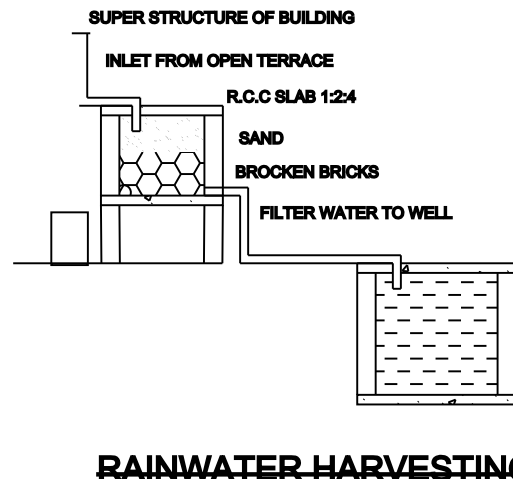
RAINWATER HARVESTING
