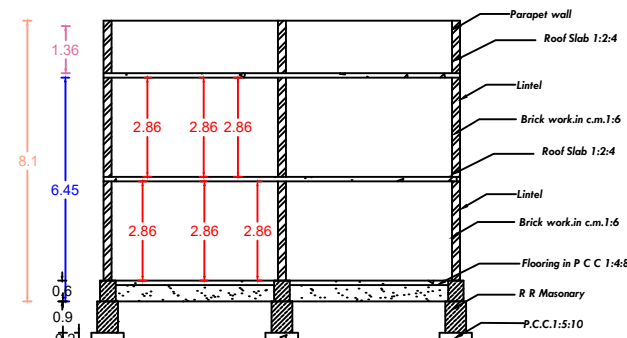
SECTION "A-B"
