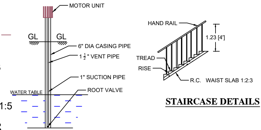
SEC. OF BOREWELL
