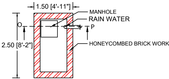
PLAN RAIN WATER HARVESTING
