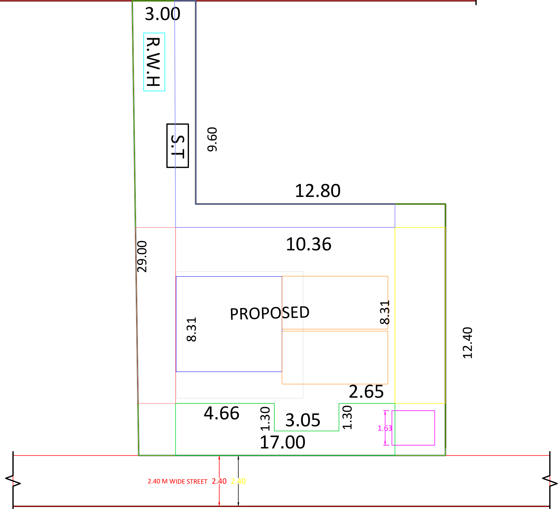
SITE PLAN
