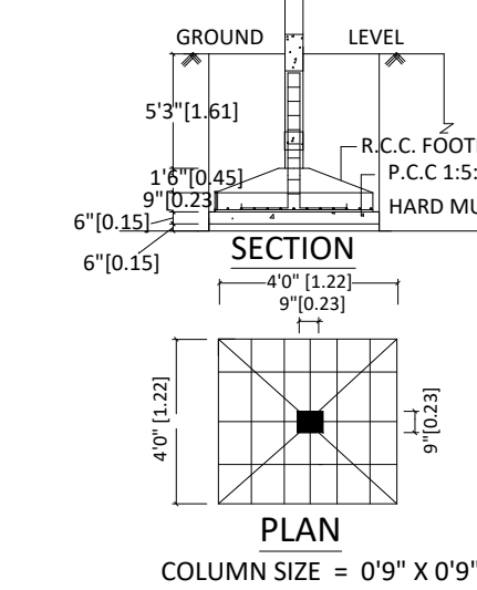
FOUNDATION DETAILS
