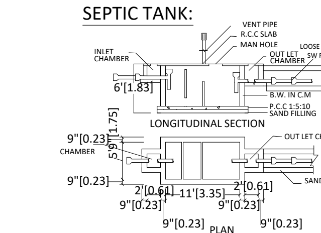
SEPTIC TANK:-
