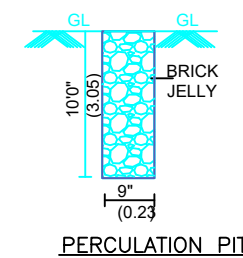
PERCULATION PIT
