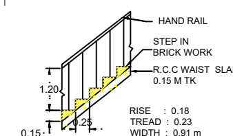
STAIR DETAILS
