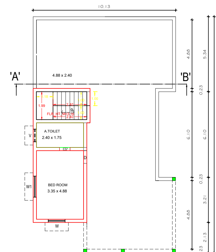
FLOOR FLOOR PLAN
