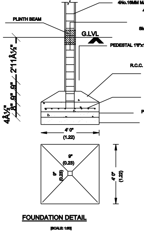
FOUNDATION DETAIL
