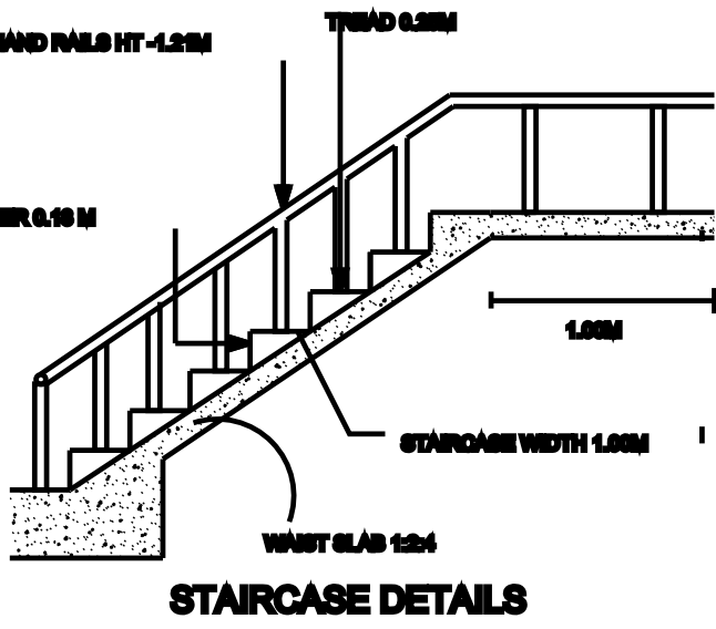
STAIRCASE DETAILS
