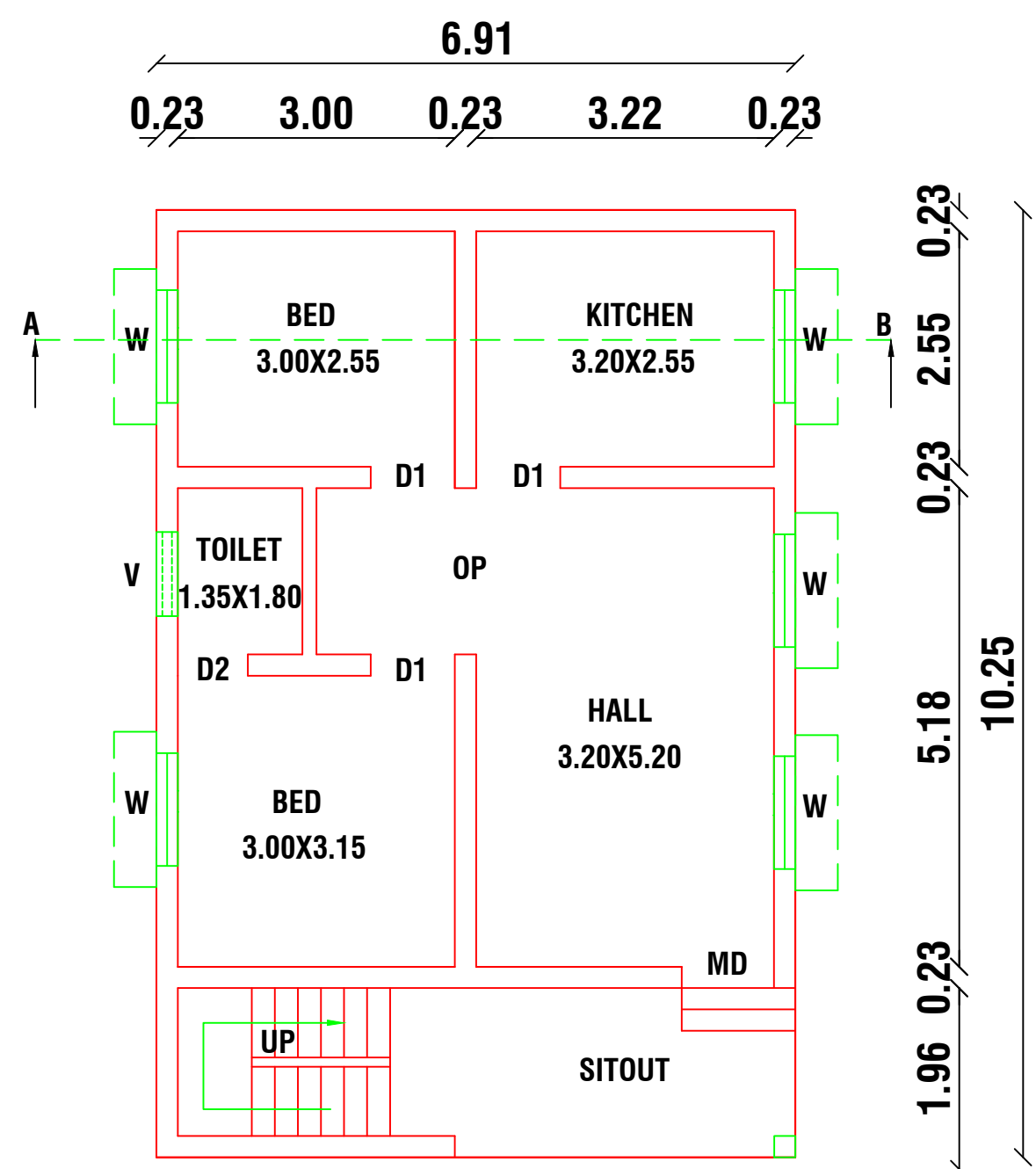
FLOOR PLAN
