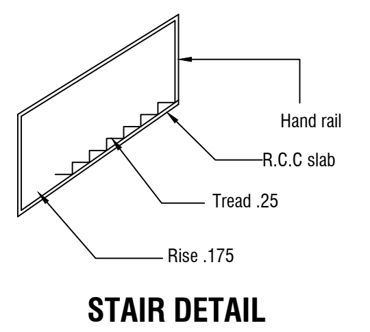
STAIR DETAIL
