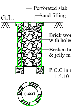
PERCOLATION PIT (NOT FOR SCALE)
