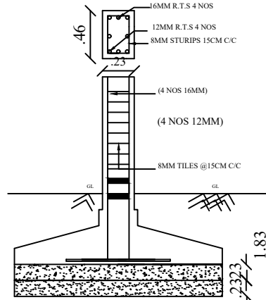
RCC COLUMN DETAILS
