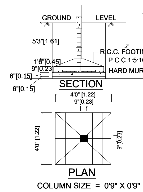
FOUNDATION DETAILS
