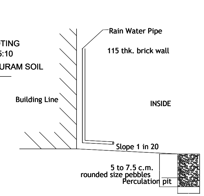
PERCOLATION PIT
