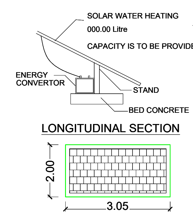
SOLAR SYSTEM
