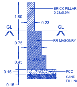
FOOTING DETAILS
