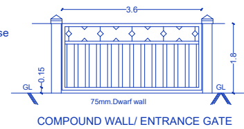
COMPOUND WALL/ ENTRANCE GATE
