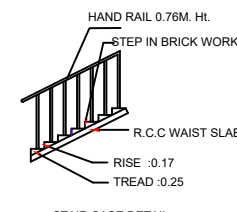
STAIR CASE DETAIL
