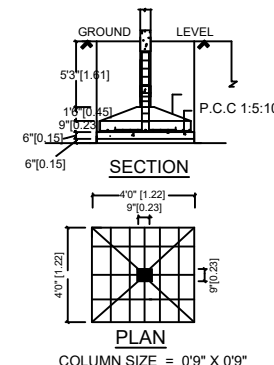
FOUNDATION DETAILS
