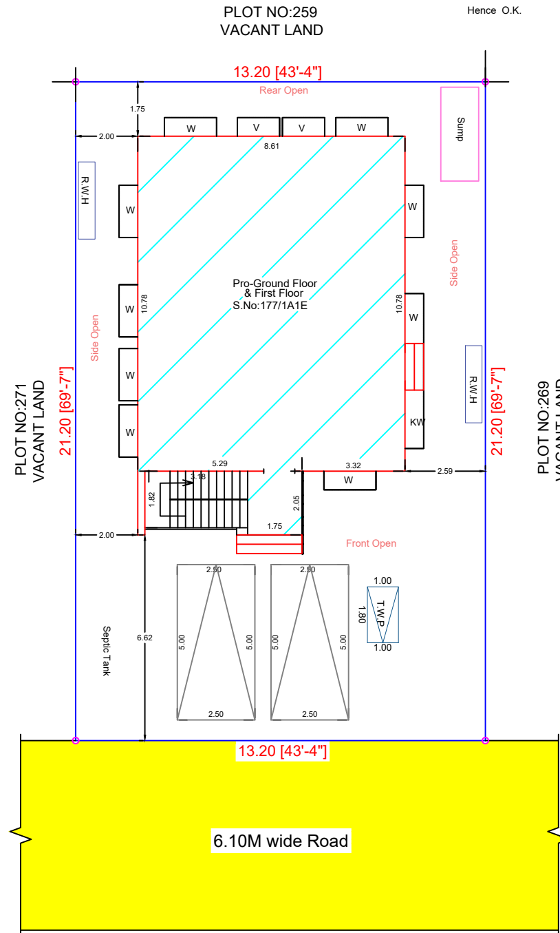
SITE PLAN (Scale 1 in 100)
