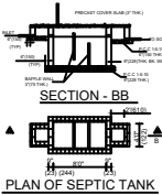
PLAN OF SEPTIC TANK
