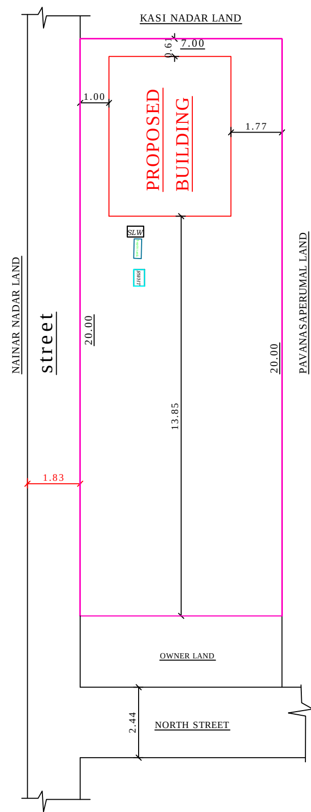
SITE PLAN
