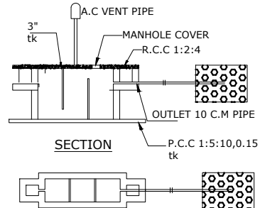
PLAN OF SEPTIC TANK & TRENCH
