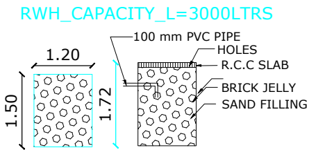
PLAN & SECTION OF RAINWATER COLLECTION TANK
