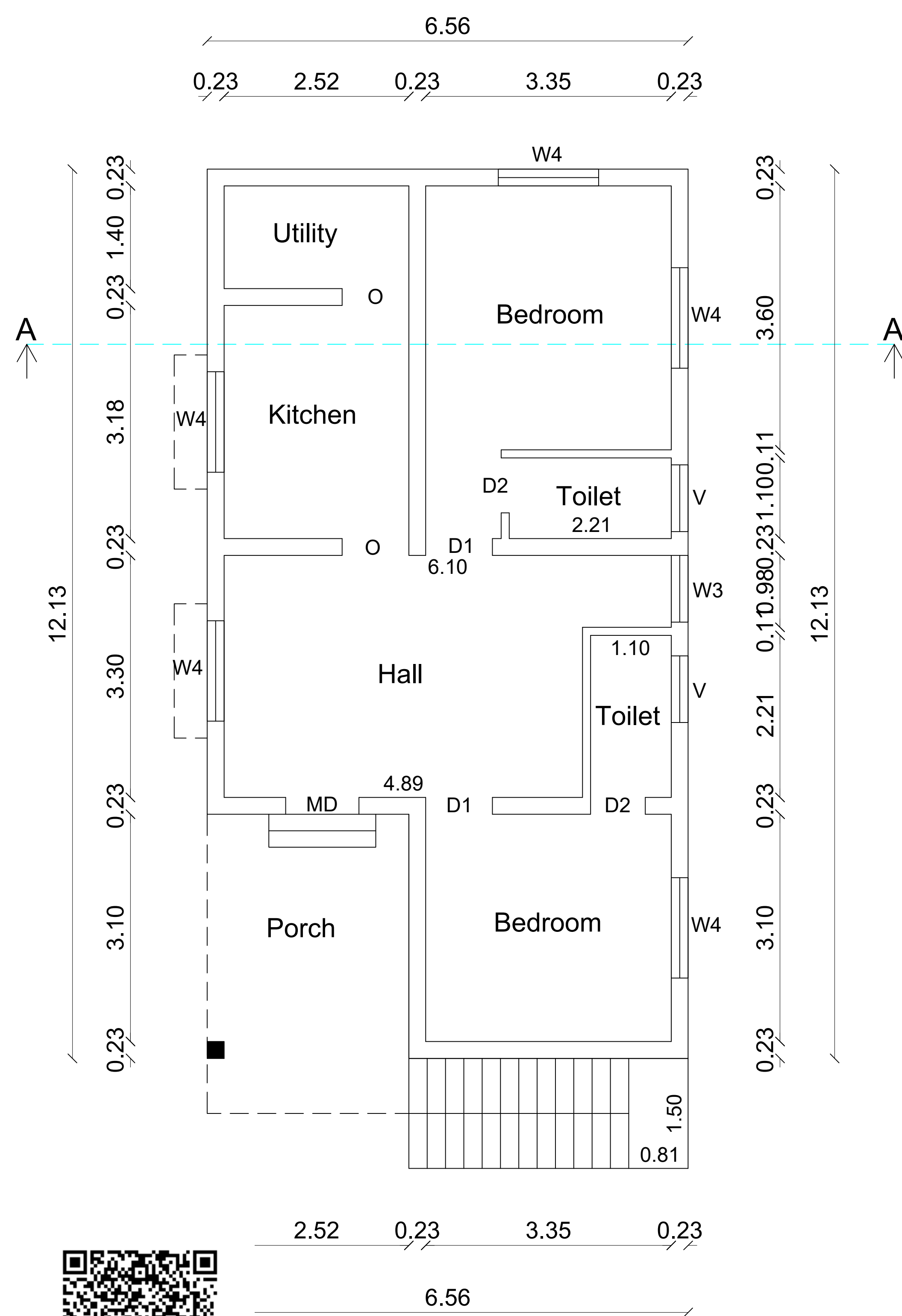
PLAN
