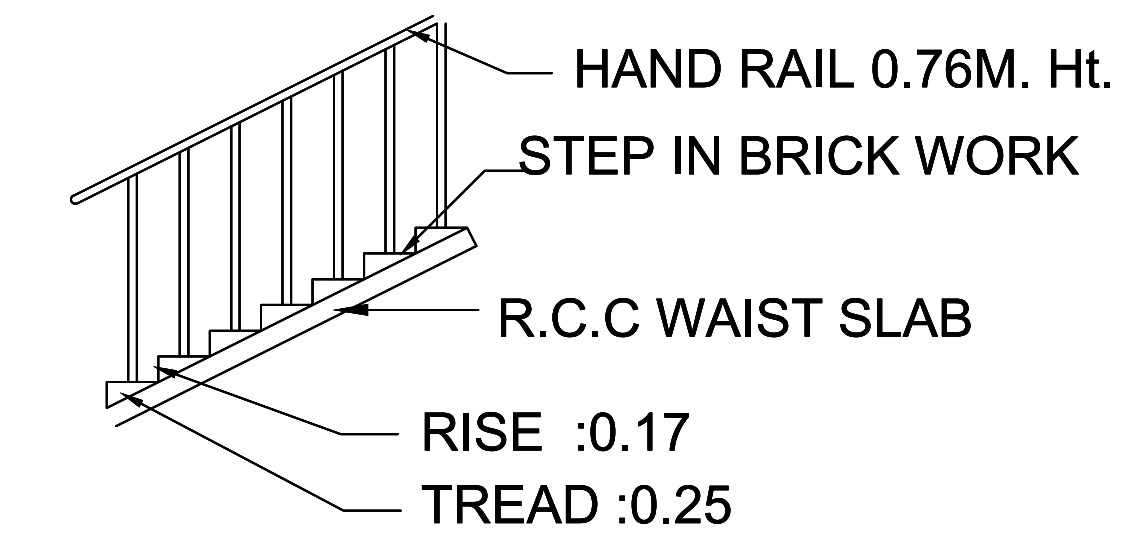
STAIR CASE DETAIL
