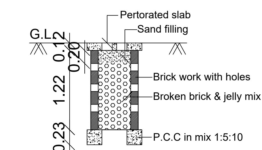
PERCOLATION PIT FOR 30 Sq. m. (Scale:- 1:50)
