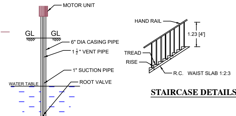
SEC.OF BOREWELL
