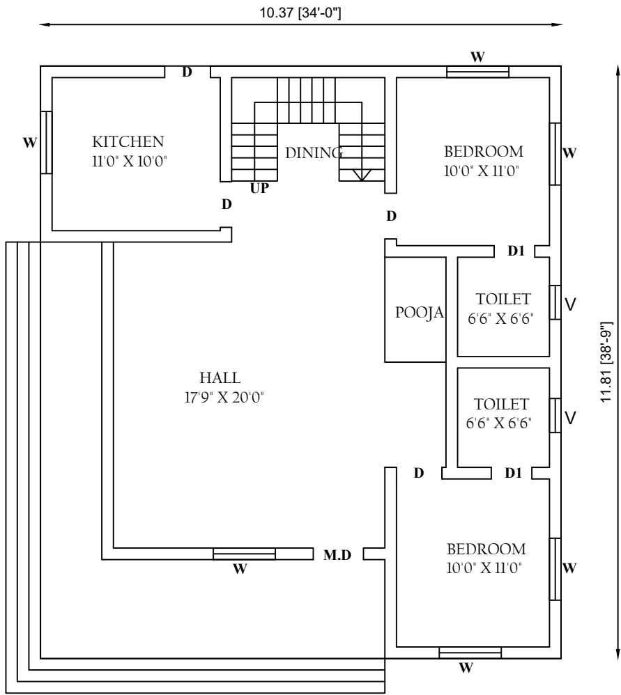
R PLAN
