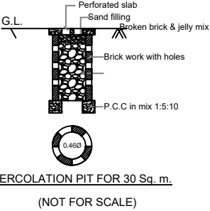
RAINWATER HARVESTING
