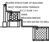
RAINWATER HARVESTING
