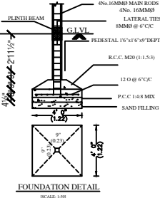
FOUNDATION DETAIL
