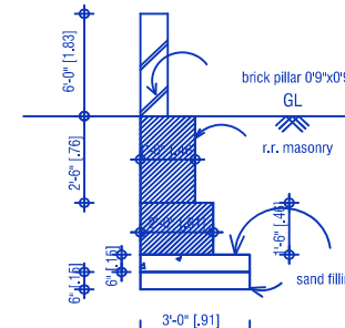
PERCOLATION PIT
