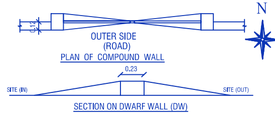
SECTION ON DWARF WALL (DW)
