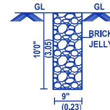
PERCOLATION PIT
