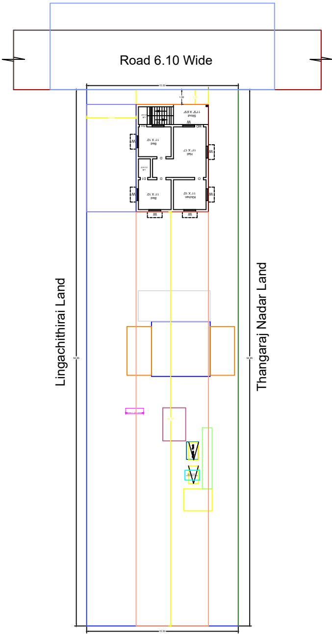
SITE PLAN
