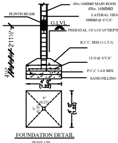
FOUNDATION DETAIL
