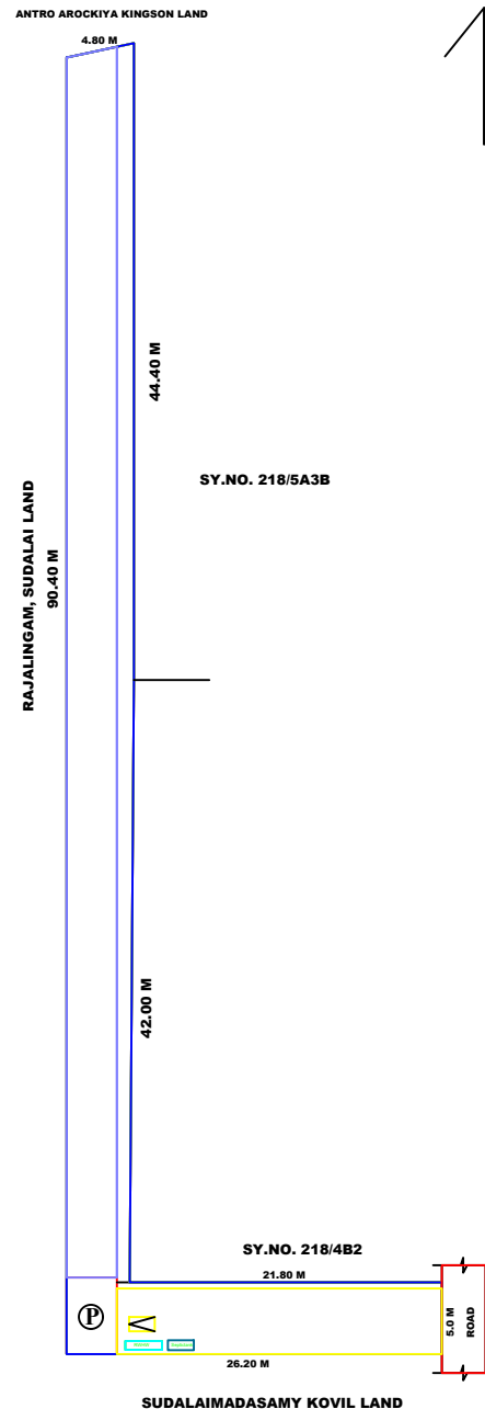
SITE PLAN
