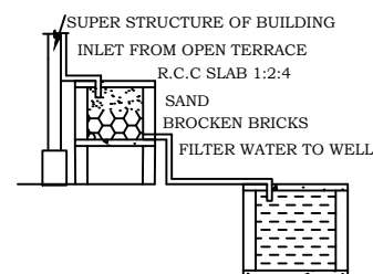
RAINWATER HARVESTING
