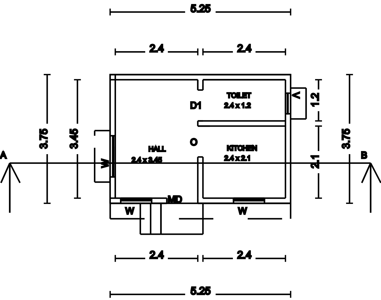
PLAN
