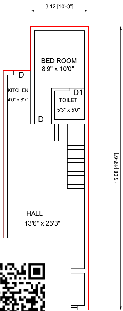
FLOOR PLAN
