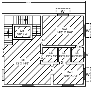
RST FLOOR PLAN
