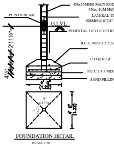
FOUNDATION DETAIL
