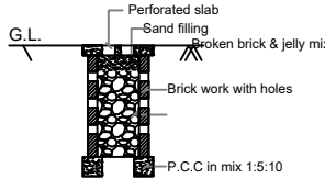
RAINWATER HARVESTING
