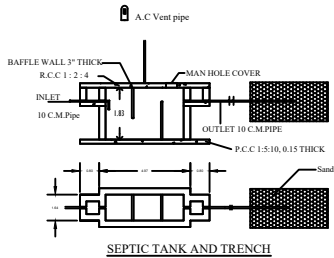
SEPTIC TANK AND TRENCH
