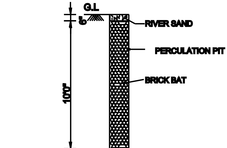
PERCOLATION PIT
