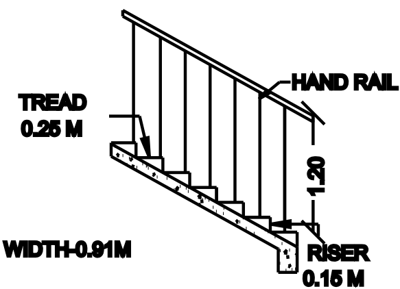
STAIRCASE DETAILS
