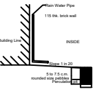
PERCOLATION PIT
