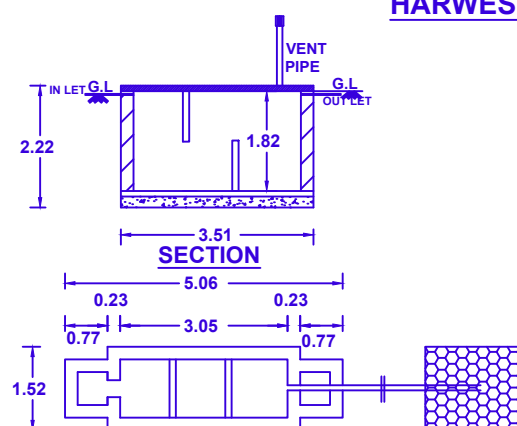
PLAN OF SEPTIC TANK AND TRENCH DETAILS
