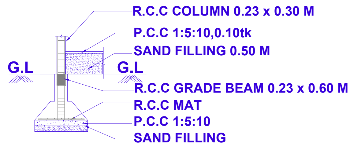
R.C.C COLUMN DETAILS
