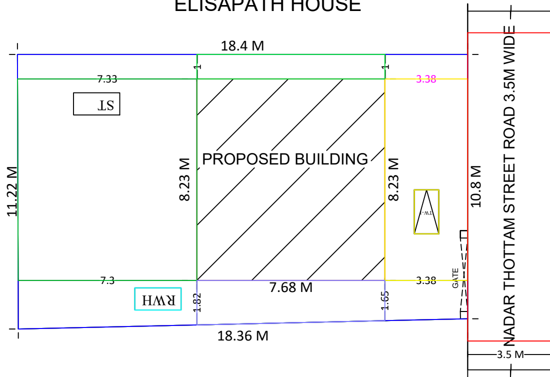
ELISAPATH HOUSE
