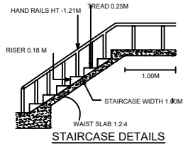
STAIRCASE DETAILS
