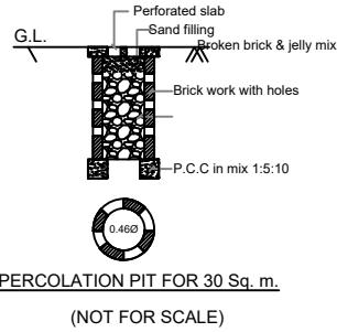
RAINWATER HARVESTING
