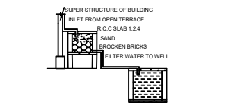
RAINWATER HARVESTING
