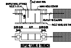
REPTIC TANK & TRENCH
