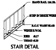
STAIR DETAIL
