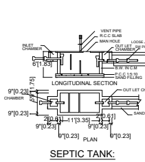
SEPTIC TANK:
