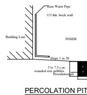
PERCOLATION PIT
