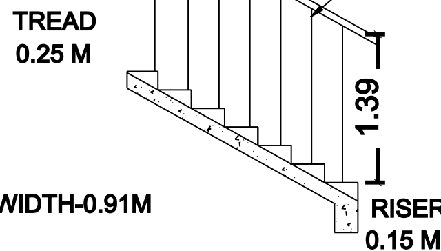
STAIRCASE DETAILS
