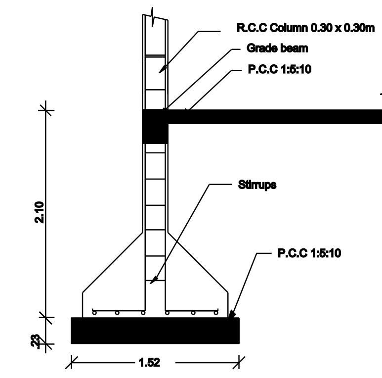
Column Detail
