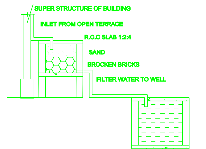
Rainwater harvesting
