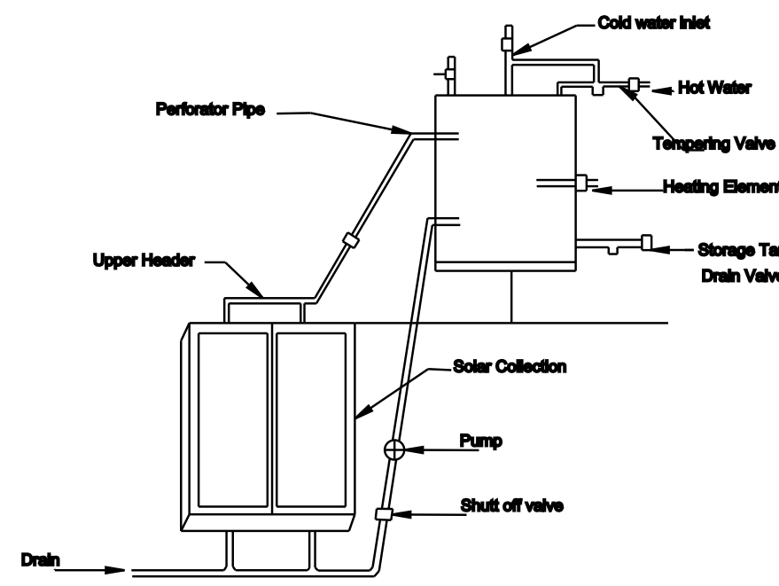
Details Of Solar Water Heater (NTS)
