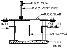
SEC. OF SEPTIC TANK
