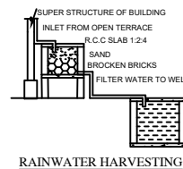
RAINWATER HARVESTING
