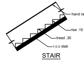
STAIR
