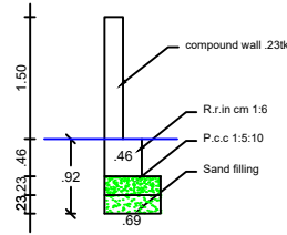
Compound wall Detail
