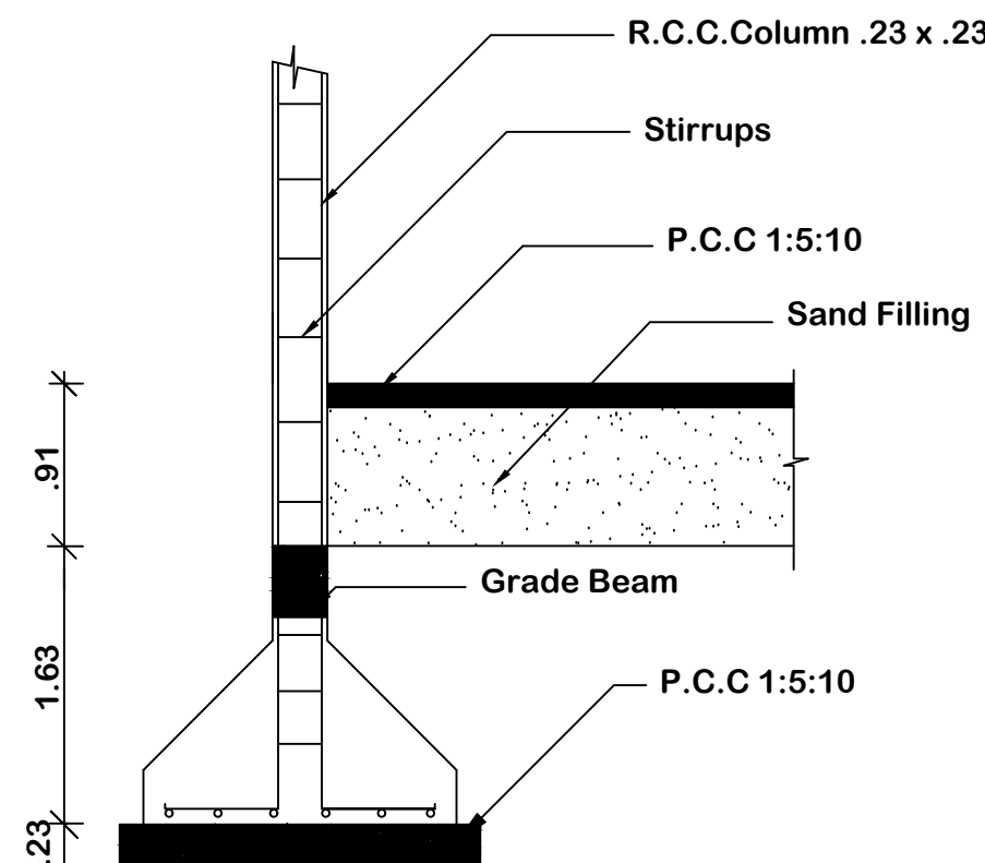
COLUMN DETAIL
