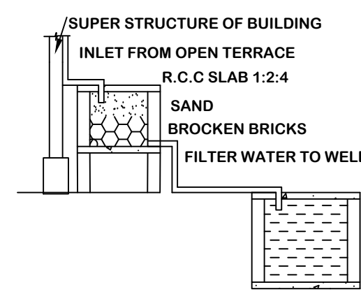
RAINWATER HARVESTING
