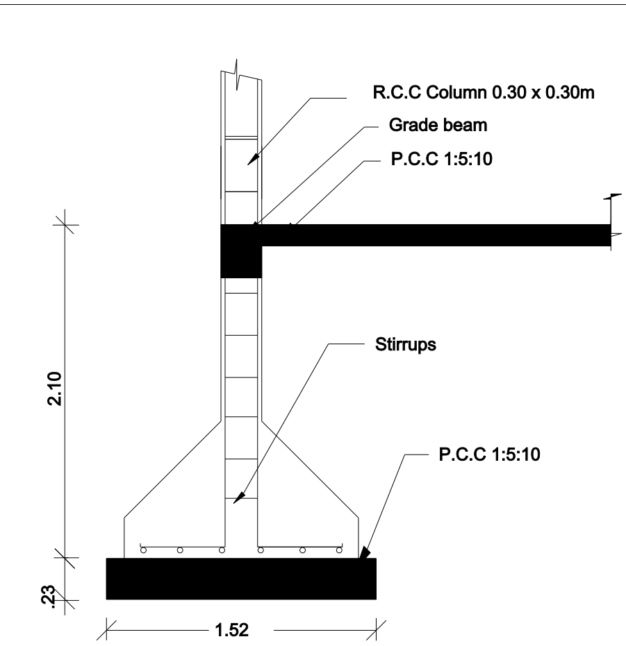
Column Detail
