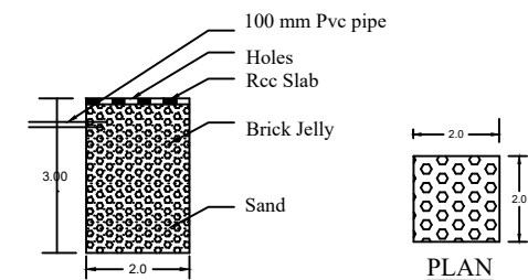
SECTION OF RAIN WATER COLLECTING TANK
