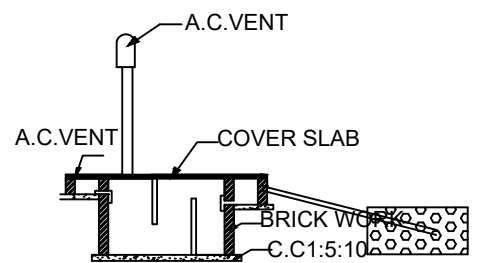
SECTION OF RAIN WATER COLLECTING TANK
