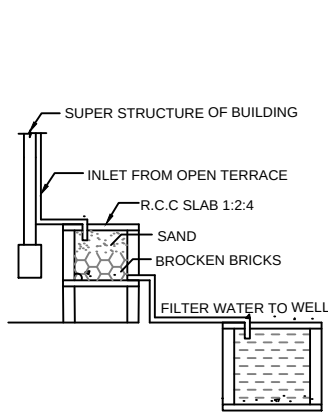
DETAILS OF FILTER BED & WELL NTS
