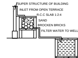
Rainwater harvesting
