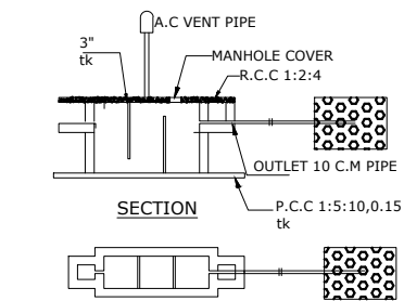
PLAN OF SEPTIC TANK & TRENCH
