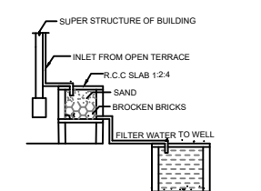
DETAILS OF FILTER BED & WELL N.T.S
