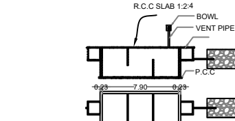
SEPTIC TANK AND TRENCH NTS
