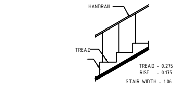
STAIRCASE DETAILS NTS
